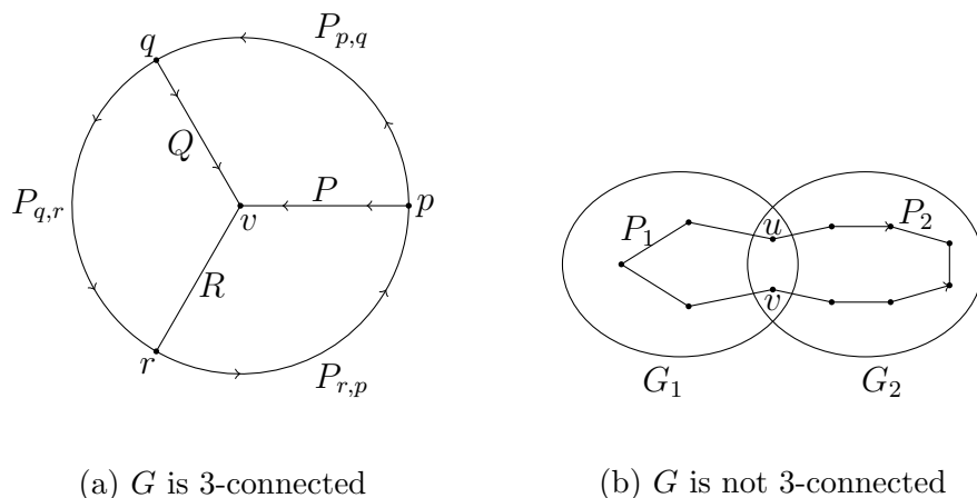
Figure 1: The two cases considered in the proof
