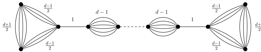
Figure 2: The padded paddle graph PP_{d,n} .
