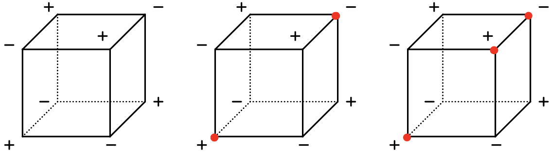
Figure 3: Left: A cuboid with \pm 1 weights labeled. Middle and right: Two cuboids, \Delta and \Delta' , with points in A labeled in red. The middle cuboid is ‘balanced’, as it satisfies A[\Delta] = 0 . The right cuboid is ‘unbalanced’, with A[\Delta'] > 0 .
