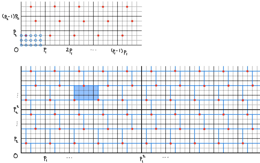
Figure 2: Top: An integer cube tiling \mathbb{Z}_M = A \oplus B for M = p_1^2 p_2^2 = 5^2 \cdot 3^2 . Here \mathbb{Z}_M is represented as \mathbb{Z}_{p_1^2} \times \mathbb{Z}_{p_2^2} , with A marked in red and B marked in blue. Bottom: The corresponding \mathcal{L}_M -periodic tiling of \mathbb{R}^2 by translates of R = [0, p_1] \times [0, p_2] . One of the translates is shaded.
