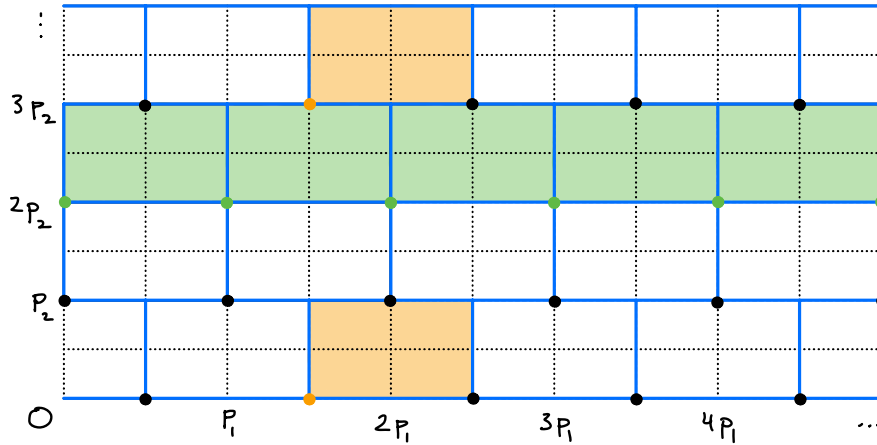
Figure 4: A tiling S \oplus R = \mathbb{R}^2 with S \subseteq \frac{p_1}{2}\mathbb{Z} \times \frac{p_2}{2}\mathbb{Z} . The dots represent points in S . The subset S_{1,\frac{3}{2}} is marked in orange, and the subset S_{2,2} is marked in green.
