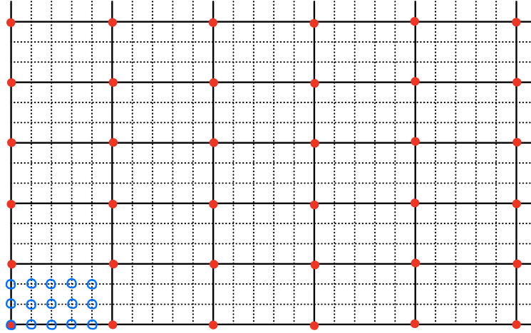
Figure 1: The sets \mathcal{L}_M (red) and \Lambda_M (blue) for M = 5 \cdot 3 .
