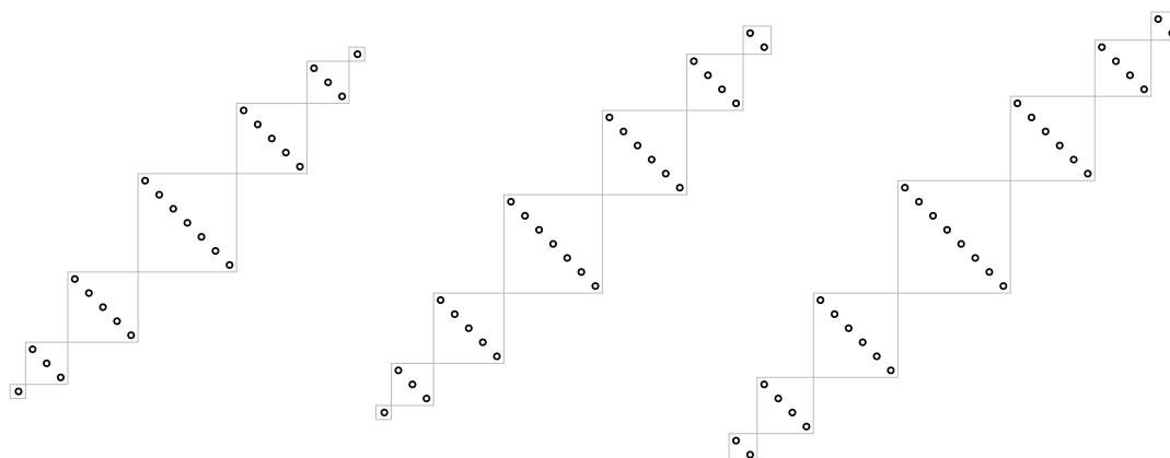
Figure 3: W[1, 3, 5, 7, 5, 3, 1] and W[1, 3, 5, 7, 6, 4, 2] and W[2, 4, 6, 8, 6, 4, 2] , they are conjectured to be maximum point sets without o-convex subset of size 13, 14, and 15 respectively. Hence N_o(13) \geq 26 , N_o(14) \geq 29 , N_o(15) \geq 33 . We also know N_o(13) \leq 27 , N_o(14) \leq 29 , N_o(15) \leq 35 .
