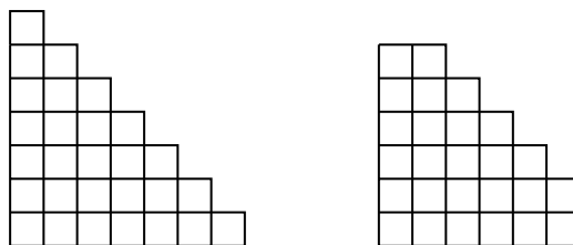
Figure 2: The triangular shape with \binom{s+1}{2} cells is extremal for n = 2s . The extremal shape for odd n = 2s - 1 is the truncated triangular shape with \binom{s+1}{2} - 2 cells. The depicted shapes have s = 7 .
