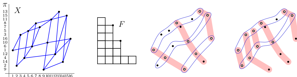
Figure 1: A point set X where the blue segments are the edges of the diagram of P = (X, <) , the Ferrers shape F = F(P) and two orthogonal pairs of X . The orthogonal pairs, with chains outlined in blue and antichains in pink, correspond to the boundary points (3, 3) and (2, 5) of F . The elements of the corresponding rectangles are emphasized.
