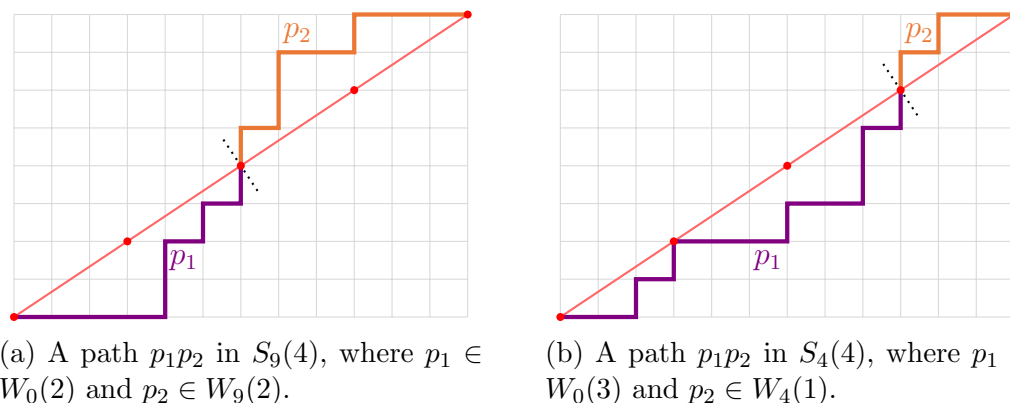
Figure 1.3: Two example min-max paths in S(4) for (a, b) = (3, 2) .
