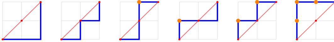
Figure 1.6: Set a = b = 1 and g = 2 . The six lattice paths from (0,0) to (2,2) are distributed as (0, 0, 1, 1, 2, 3) according to the number of lattice points above the boundary. Here W_0(2) = W_1(2) = \mu_0(2) = 2 and W_2(2) = W_3(2) = \mu_1(2) = 1 (illustrating Corollaries 1.6 and 1.8). The six lattice paths are distributed as (0, 0, 1, 1, 2, 2) according to the number of vertical steps above the boundary (illustrating the Chung–Feller result given in Theorem 1.14).
