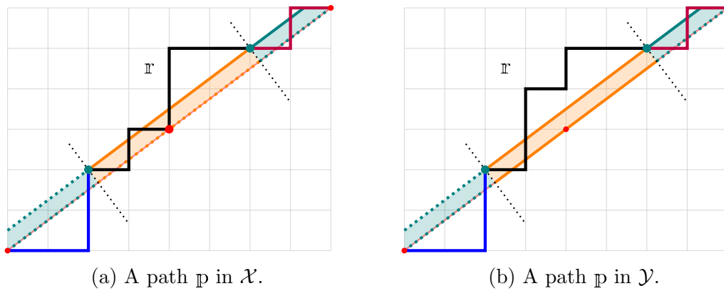
Figure 3.5: Let (a, b) = (4, 3) . In diagram (a), we have \mathbb{p} \in W_7(2) and the subpath \mathbb{r} between the (last) two LPAs of \mathbb{p} contains a boundary point of \mathbb{p} . In diagram (b), we have \mathbb{p} \in W_8(2) and the subpath \mathbb{r} between the (last) two LPAs of \mathbb{p} contains no boundary points of \mathbb{p} .
