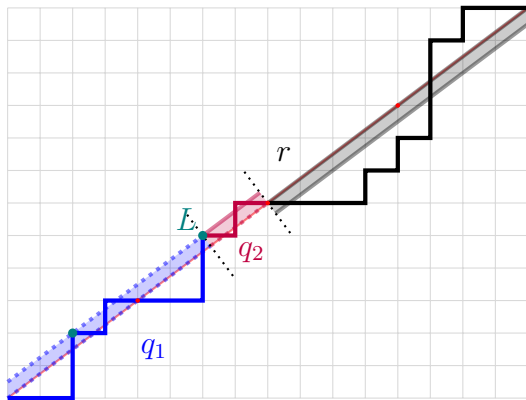
(c) Canonical representation of a path p in Y .
