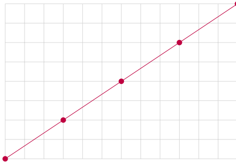
Figure 1.2: Let (a, b) = (3, 2) . The boundary of a path whose endpoint is (ga, gb) = (4 \cdot 3, 4 \cdot 2) contains g + 1 = 5 lattice points (red vertices).
