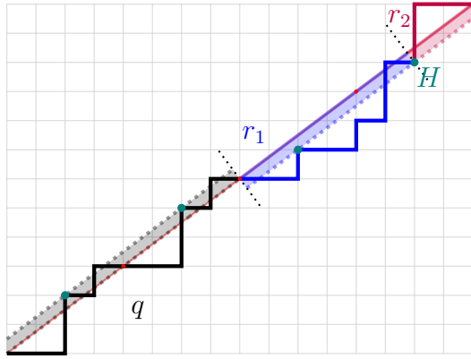
(a) Canonical representation of a path p in X .
