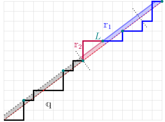
(b) Canonical representation of a path p in X .
