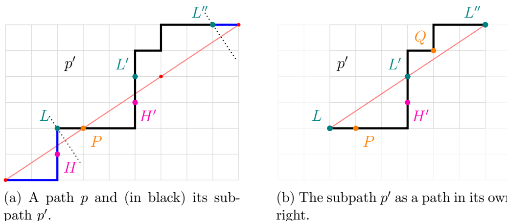
Figure 3.2: Let (a, b) = (3, 2) . The path p is a member of W_7(3) \setminus S_7(3) containing the interior boundary point P and the LPAs L, L', L'' and HPBs H, H' . The subpath p' contains the same interior boundary point and LPAs as p , as well as the HPB H' of p . The path p' (on its own) has the same slope as p , but is a member of S_4(2) \subseteq W_4(2) containing the boundary points L, L', L'' , the unique HPB P , and the unique LPA Q . We note that H' is not an HPB of the path p' .
