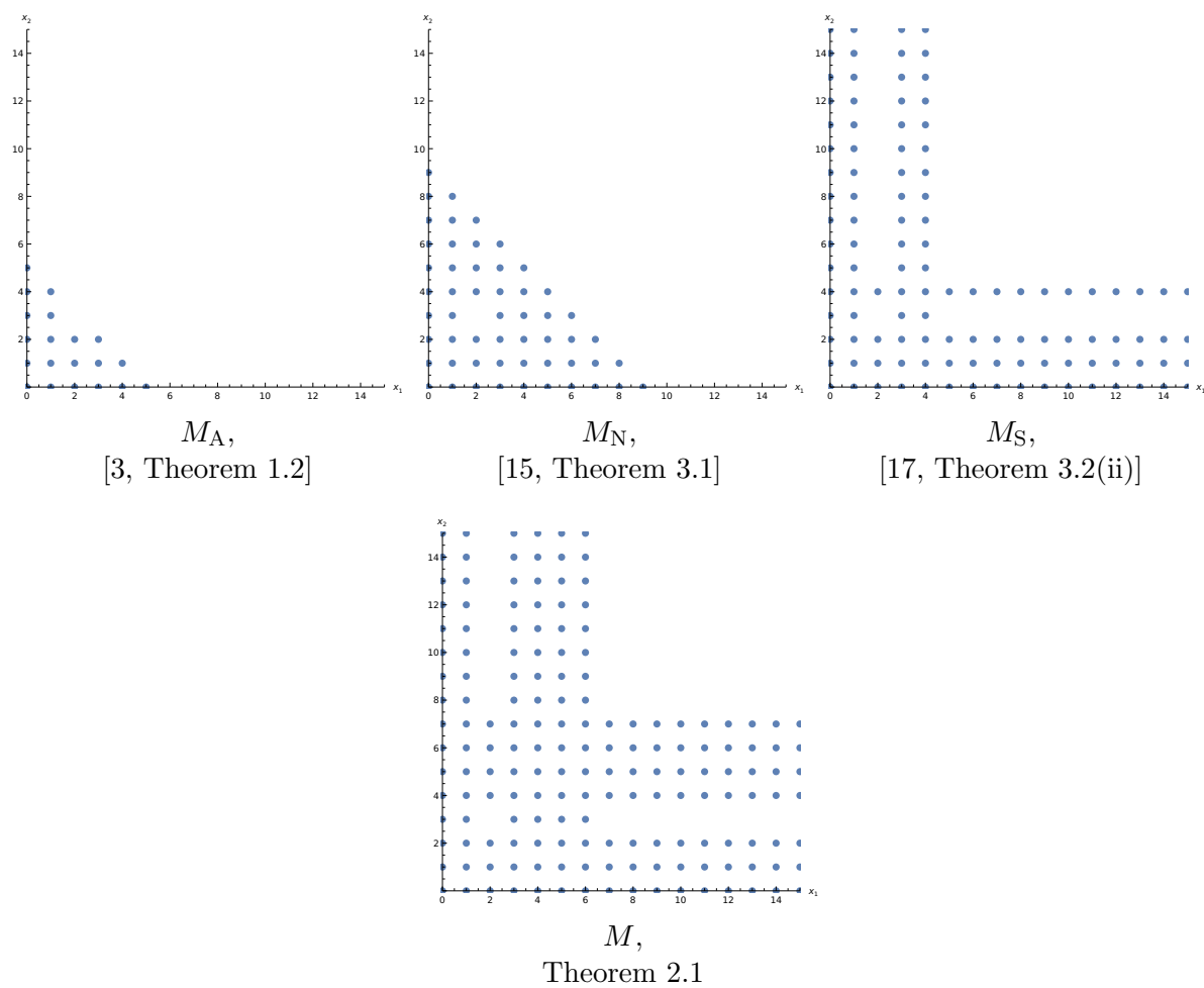
Figure 1: x_1^2x_2^3 + any linear combination of the dotted monomials does not vanish on S = \{(x_1, x_2) \in \mathbb{C}^2 \mid x_1^5 = x_2^5 = 1\} .
