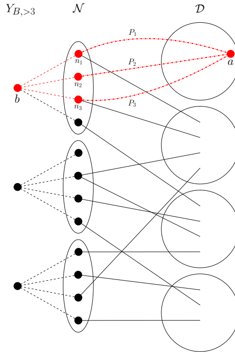
Figure 5: An illustration of the theta that appears in H when H'' has maximum degree at least 9.
