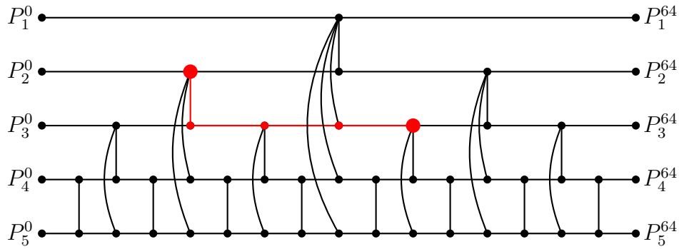
Figure 3: A nonstandard path between two (enlarged) big vertices
