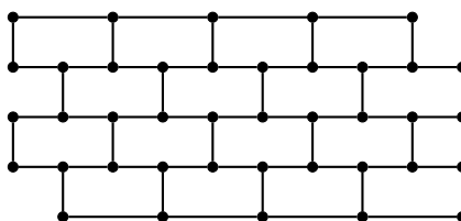
Figure 1: W_{5 \times 5}
