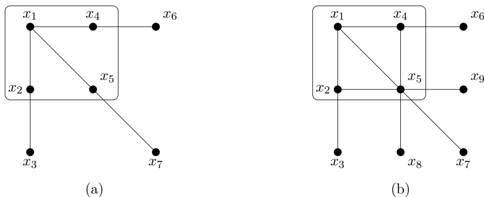
Figure 11: The triangles in Lemma 3.8. In each case, \{x_1, x_2, x_4, x_5\} is a 4-cocircuit.
