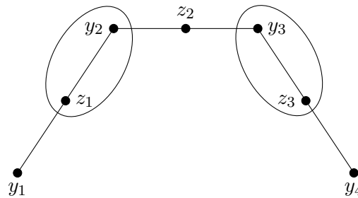
Figure 14: \{z_1, y_2, y_3, z_3\} is a 4-cocircuit in Lemma 32 and this pattern continues.
