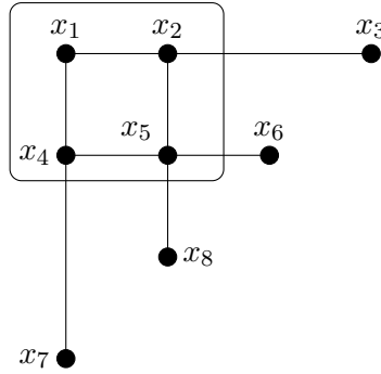
Figure 19: The triangles of M at the beginning of the proof of Lemma 35.
