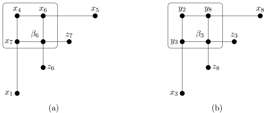
Figure 22: The symmetry between two cases in Lemma 35.
