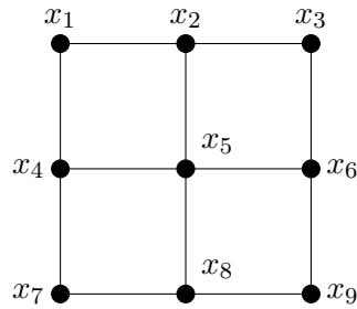
Figure 5: Some 3-point lines in a rank-4 matroid.
