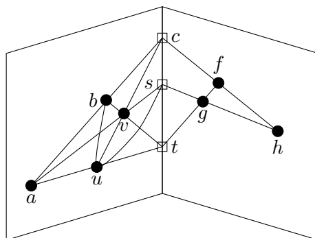
Figure 3: The labels of F_7^* used in Theorem 11.
