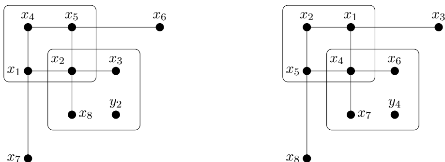
Figure 20: The outlined sets correspond to cocircuits.
