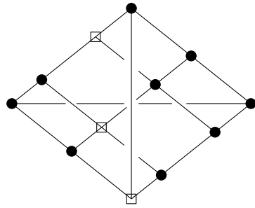
Figure 2: The rank-4 ternary affine matroid Q_9 and the matrix A , where [I_4|A] is a ternary representation of Q_9 .
