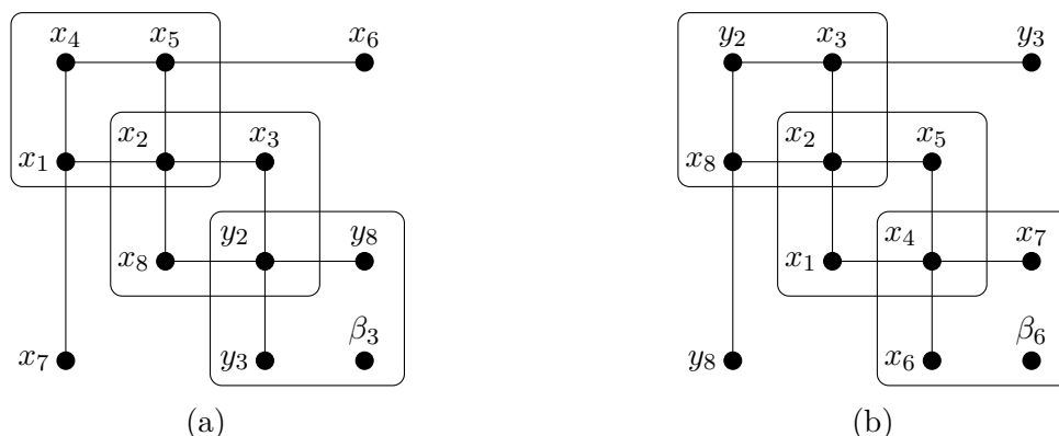
Figure 23: The cocircuits include the outlined sets along with \{x_5, x_6, x_8, y_8\} or \{x_1, x_3, x_7, y_3\} , respectively.
