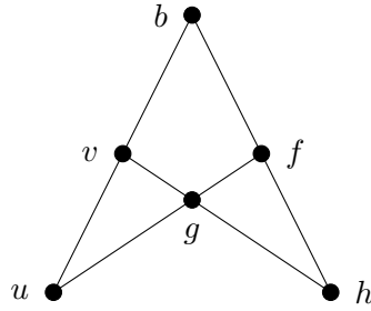
Figure 4: The matroid N \setminus e/a in Theorem 11.
