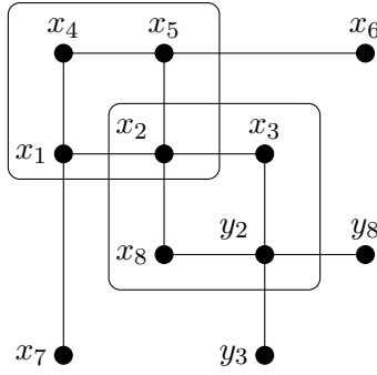
Figure 21: The outlined sets correspond to cocircuits.
